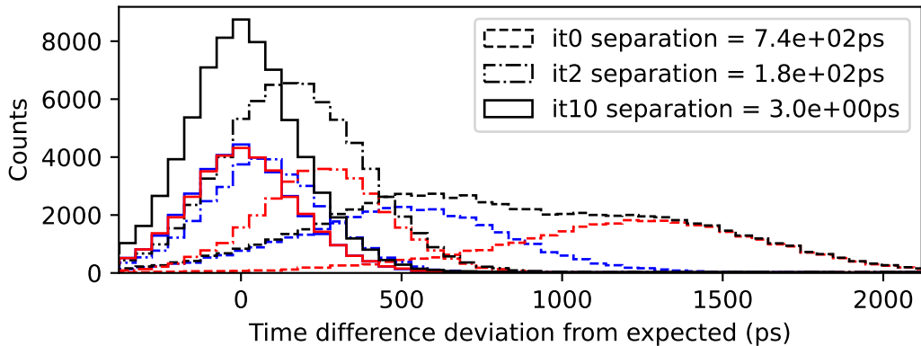
Time difference deviation from expected, channel 1951
